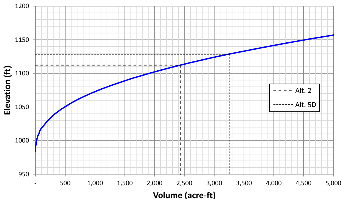
Figure 3-1. Volume-elevation curve for the Upper CWD.
